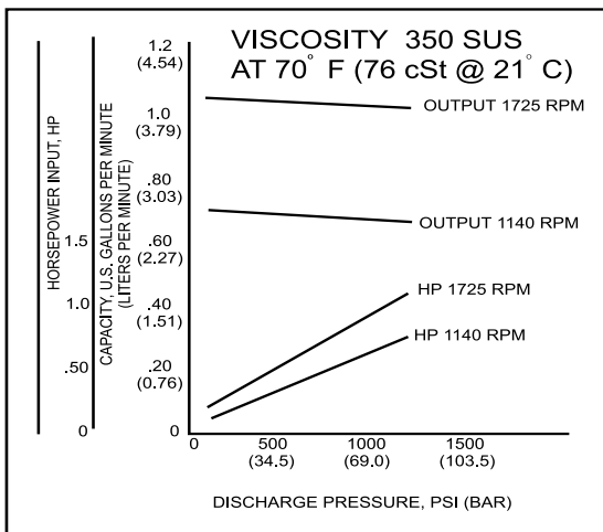
CHARTS ABOVE ARE FOR BOTH PUMP NUMBERS 557820 (540-800-111) (CCW) AND 558955 (540-800-940) (CW)
